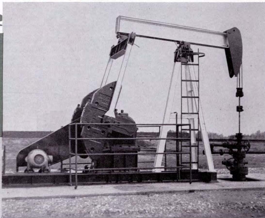
↑ LUFKIN T5α-80D UNIT. Texaco Exploration Company, Redwater Field.
