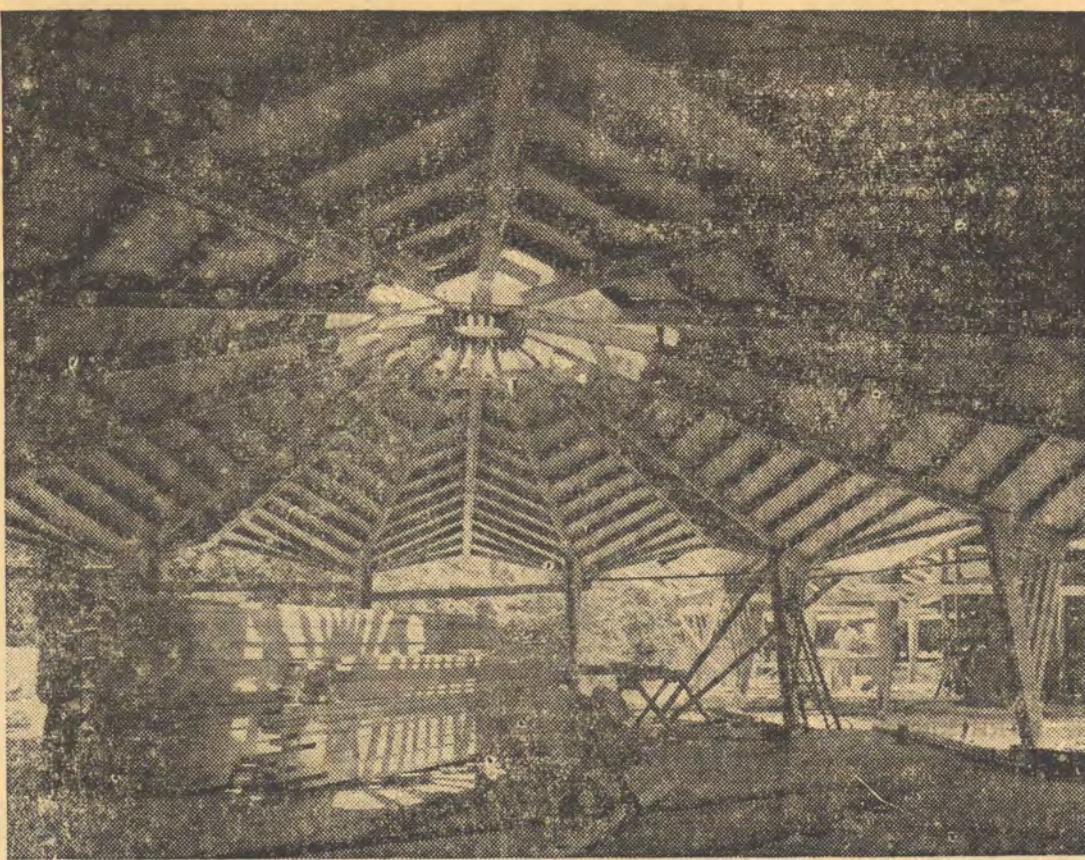
RISEING STAR —Here is star shaped house, designed by Architect Albert C. Ledner of New Orleans. A wide area was roofed in, involving less material than old methods, and rare exploitation of the natural strength of Southern Pine lumber. Key is the wood sheathing, a sort of structural skin, which ties members together. Other parts are ridge and valley members which establish triangular sections known as planes or membranes.
