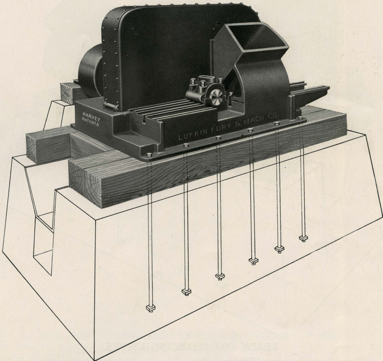
GENERAL VIEW SHOWS RIGHT HAND MACHINE.
