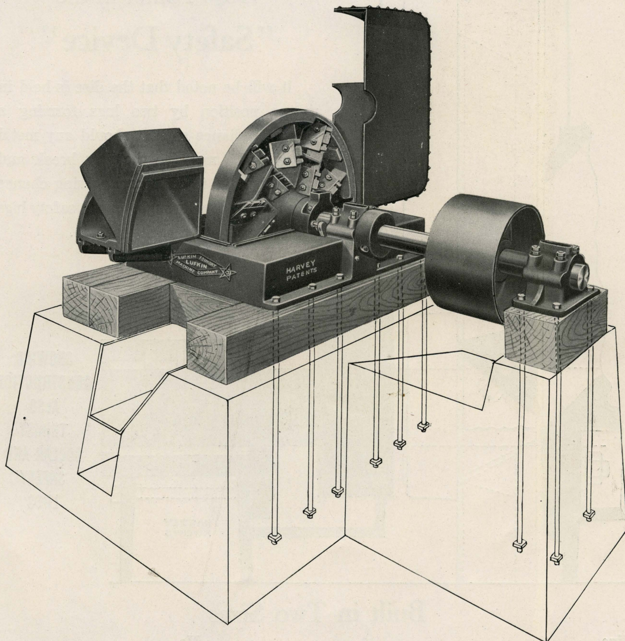
REAR VIEW SHOWING SAFETY DEVICE, ALSO SIMPLICITY OF DESIGN— ALL PARTS EASY TO GET AT, ETC.
