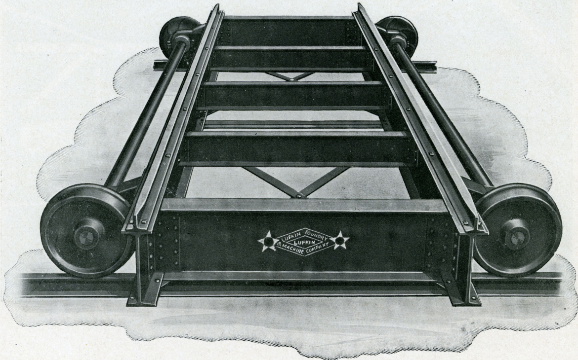
Transfer Car for Endwise Piled Dry Kiln Lumber
